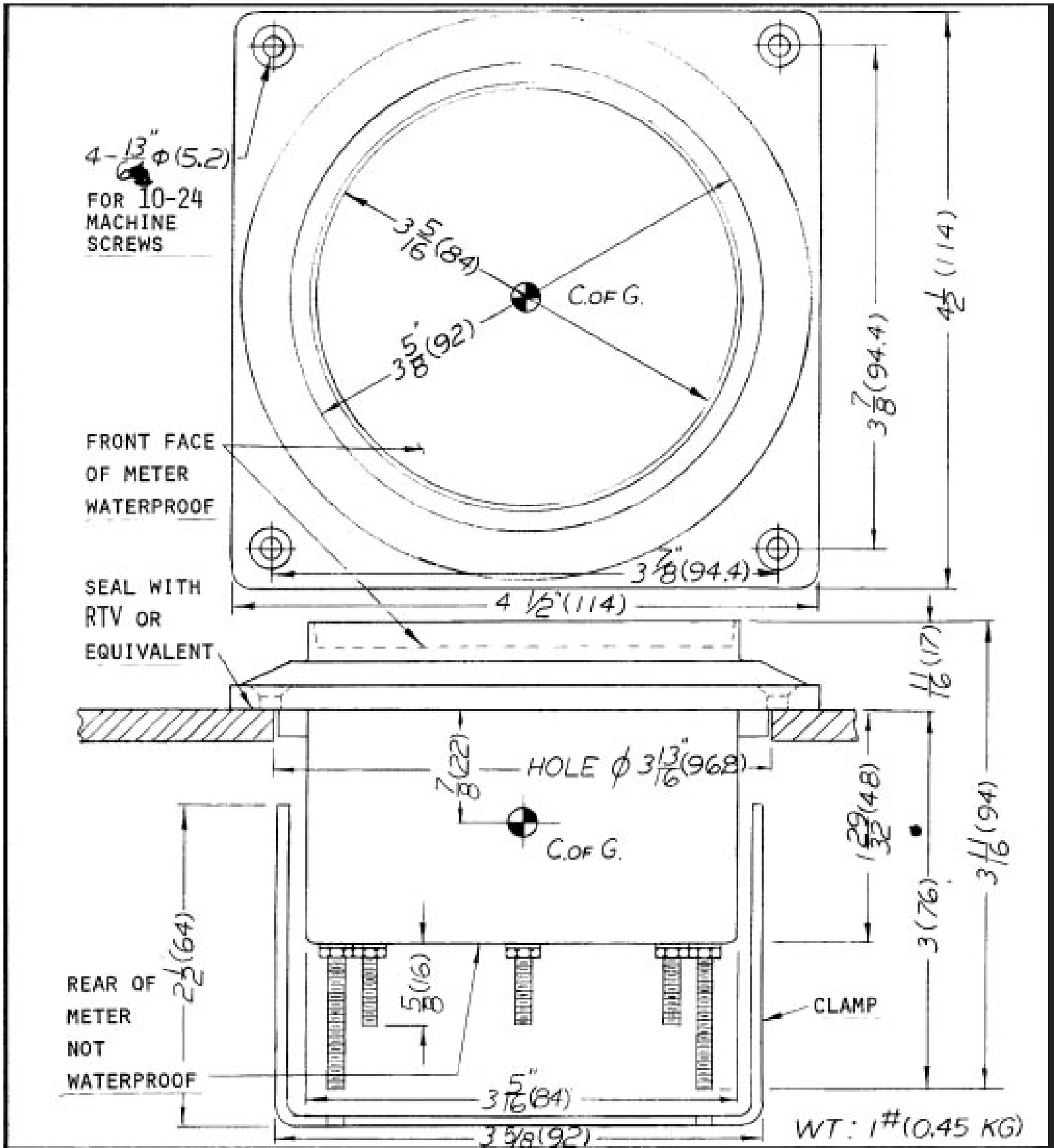
R.A.I. 150 BEZEL MOUNT - OVERALL DIMENSIONS
