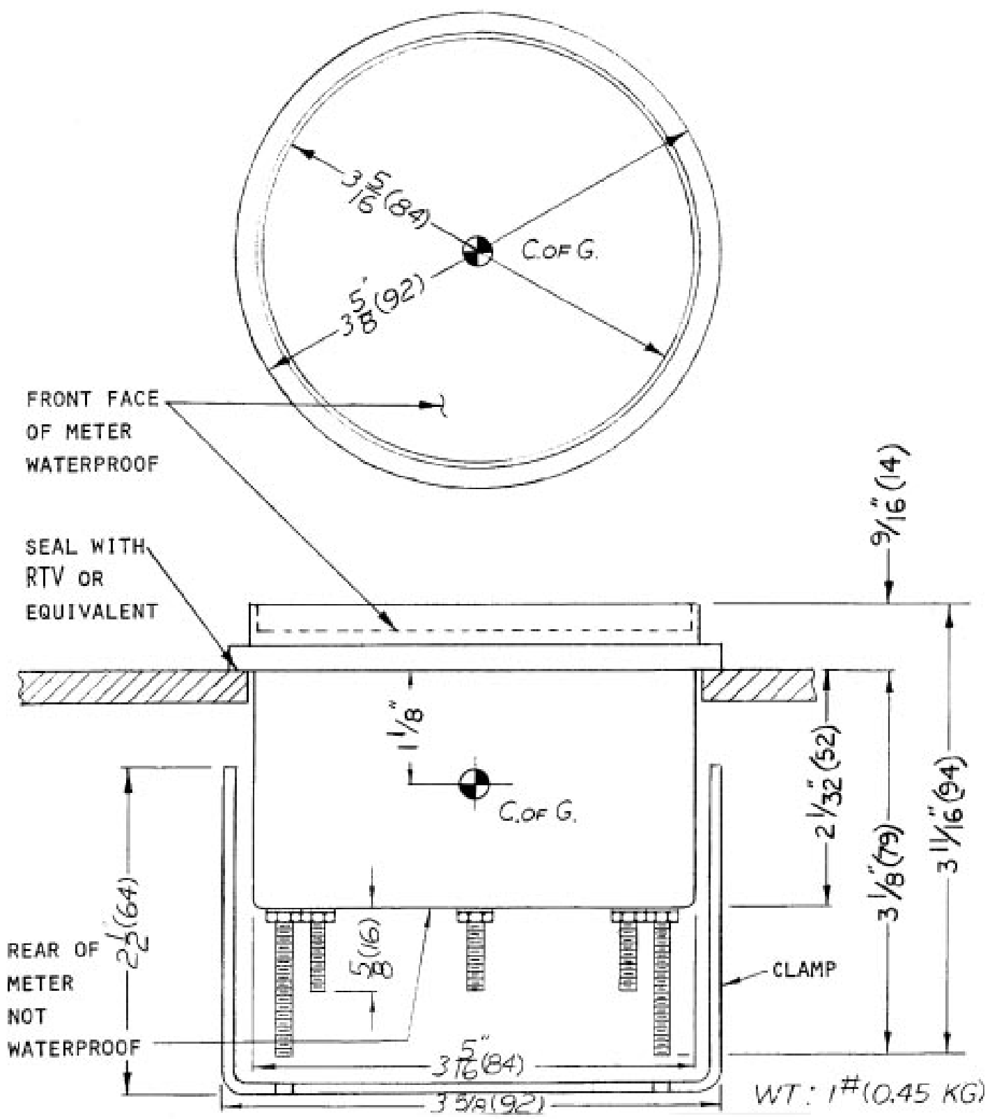
R.A.I. 150 FLUSH MOUNT - OVERALL DIMENSIONS
